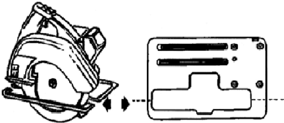
Figure 3. Builder's circular saw . Cut the foot assembly of the 10 ¼" circular saw as shown. File or grind the cut edges of the foot assembly to remove sharp edges. This size saw is necessary on Mosler or Diebold-Mosler Class 5 security files. A 7 ¼" builders circular saw is adequate for other files and does not require the modification shown above.
